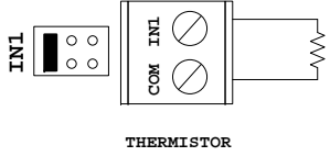
THERMISTOR
