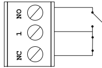
RELAY OUTPUT
