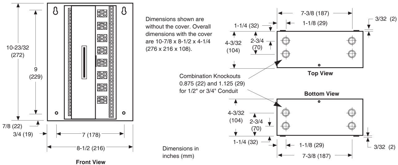
Figure-2 ENC-sLON-7-W Wall Mounting Dimensions.
