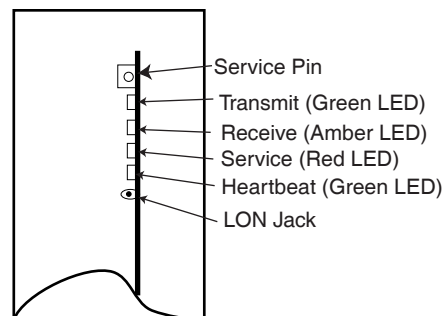
Figure-5 LED Indicators.
