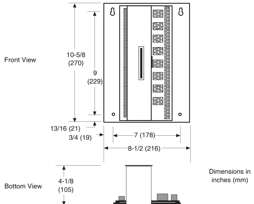
Figure-1 ENC-sLON-7-P Panel Mounting Dimensions.
